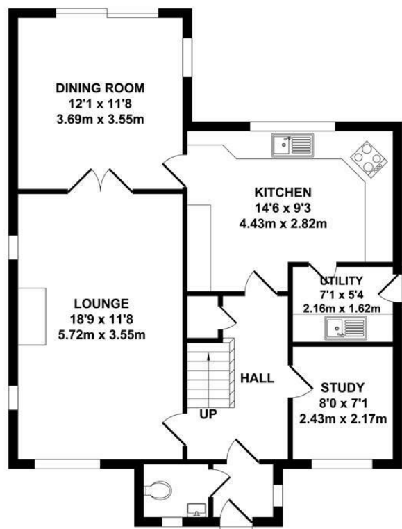
GROUND FLOOR APPROX. FLOOR AREA 746 SQ.FT. (69.27 SQ.M.)
